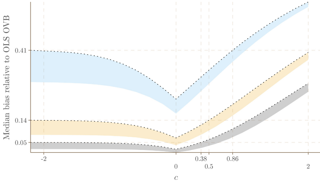
Fig. 2. Relative median bias of \hat{\beta}_{IV} conditional on t_1 > c . The figure plots median( \hat{\beta}_{IV} - \beta \mid t_1 > c )/ |\beta_{WOLS} - \beta| as a function of test cutoff c for select values of E[F] . Shaded areas cover the range of variation in relative bias over possible values of \rho . Blue: E[F] = 2 , orange: E[F] = 3.5 , gray: E[F] = 5 . Dotted lines denote limiting relative bias as \rho \rightarrow 0 . For each value of E[F] , horizontal gridlines mark the value of this relative bias when c = -\infty , and vertical gridlines mark the cutoff value for which screening on t_1 > c increases bias relative to no screening. See Appendix A.7 for computational details. (Colors appear in the online version of this article.)
