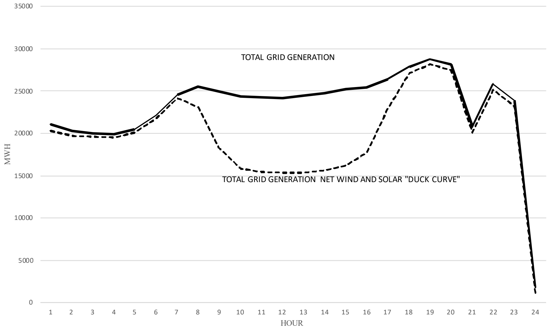
FIGURE 9 CAISO TOTAL AND NET GENERATION February 7, 2018
