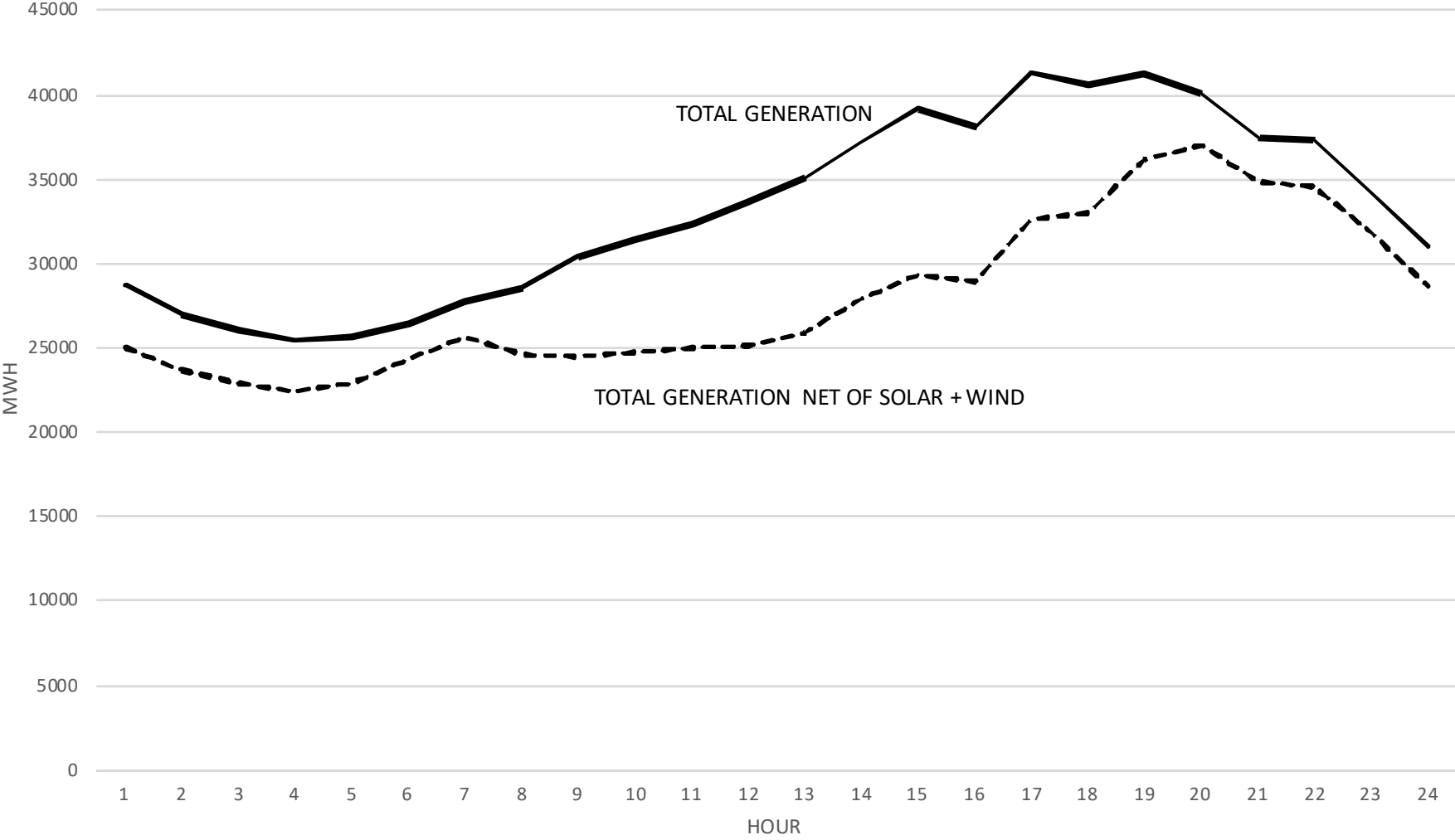
FIGURE 8 CAISO TOTAL AND NET GRID GENERATION July 18, 2018
