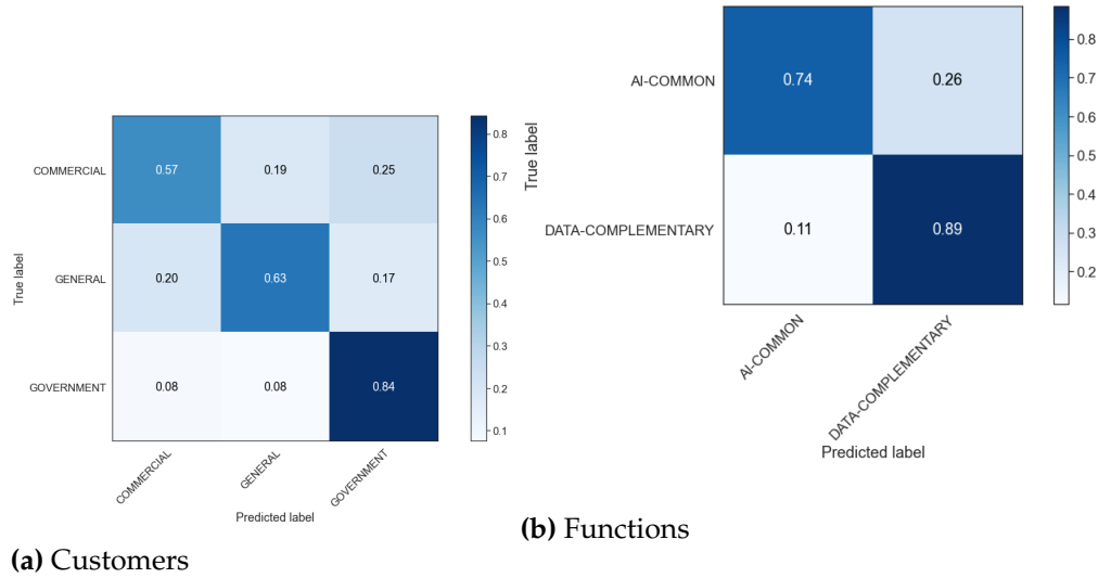
Figure A.8: Confusion matrix of categorization outcomes for software categorizations. True labels are based on training set constructed by human categorizations (performed by two individuals). Predicted labels are outputs based on Recurrent Neural Network with Long Short-Term Memory algorithm. Left panel shows categorization by customers; right panel shows categorization by function.
