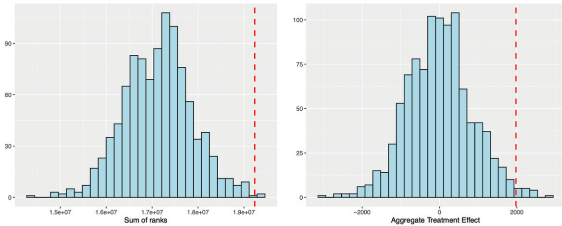
Figure 3. Permutation tests for the NSW data. Note: Results are obtained for 1000 permutations, using a fixed value of \lambda = 0.1 . The left panel displays the histogram of the sum-of-ranks statistics. The right panel displays the histogram of the aggregate treatment effect. The red dotted line is the value of the statistics for the observed assignment. p -values for the one-sided tests are 0.003 and 0.013, respectively.
