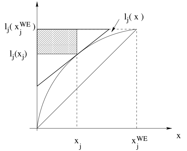
Fig. 2. Illustration of the proof of Lemma 2.
