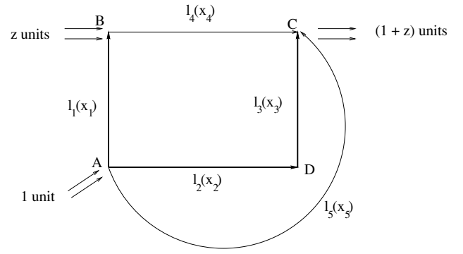
Fig. 3. A subnetwork with multiple exit points.
